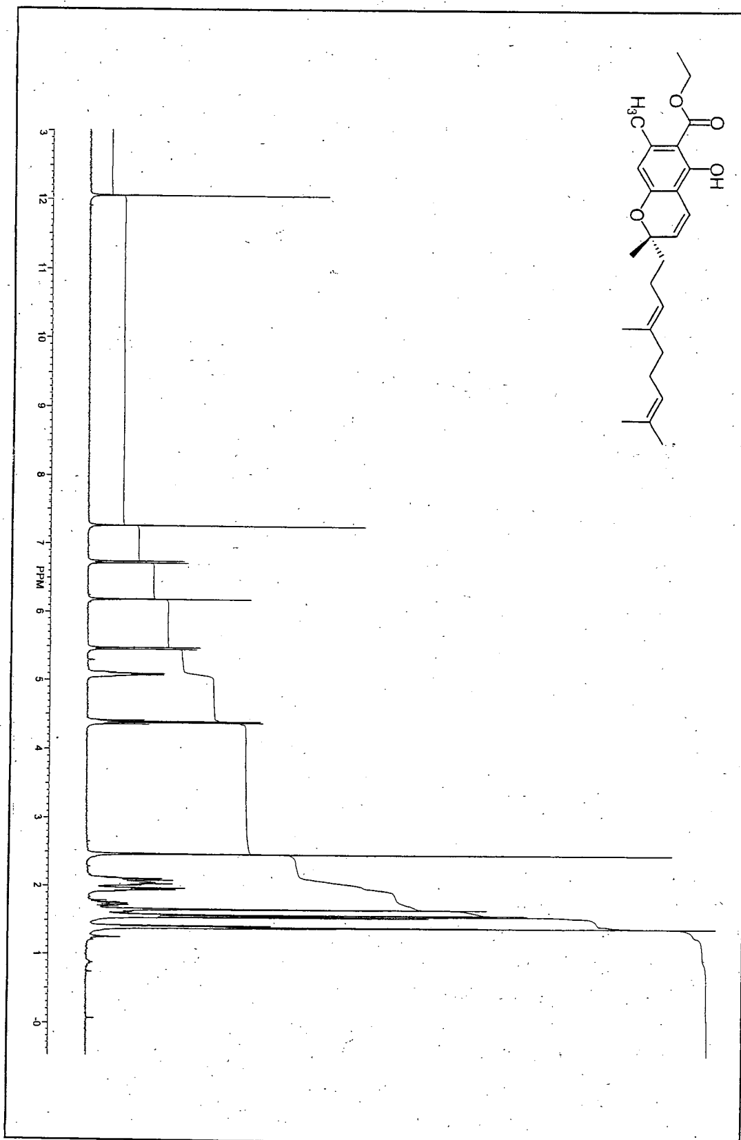
360 MHz ^1\text{H} NMR of compound 7
