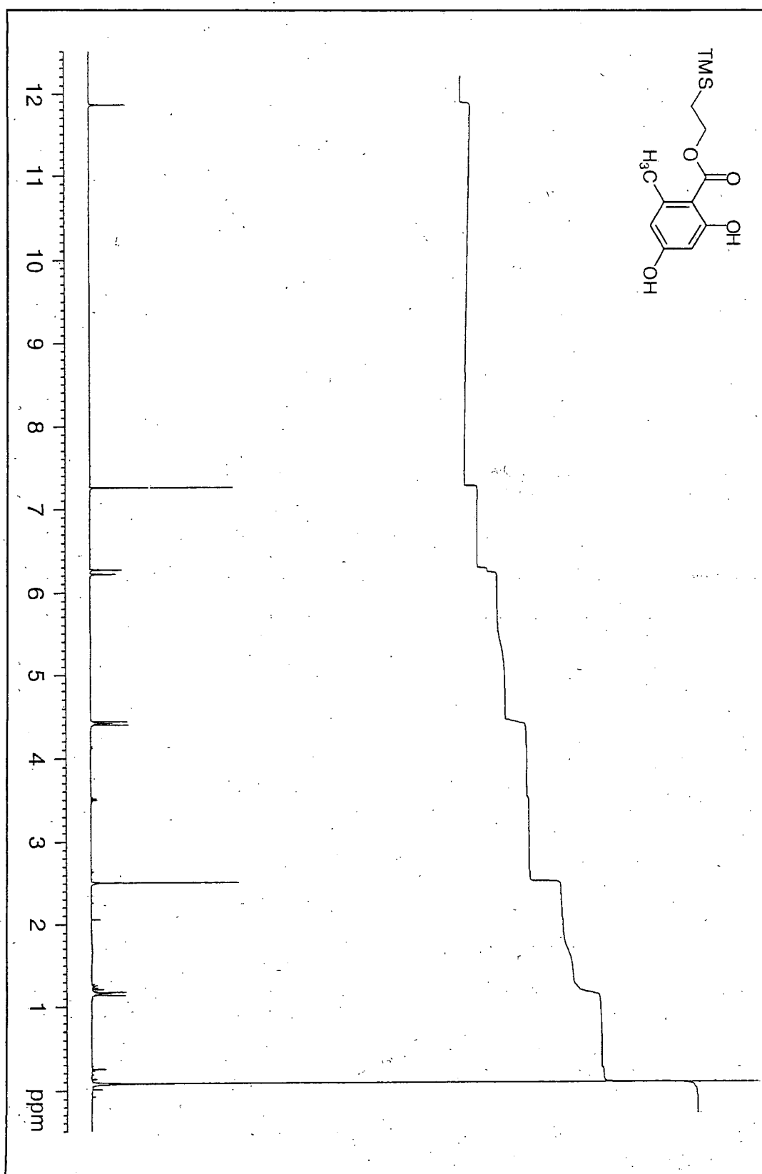
400 MHz 1 H NMR of compound 11
